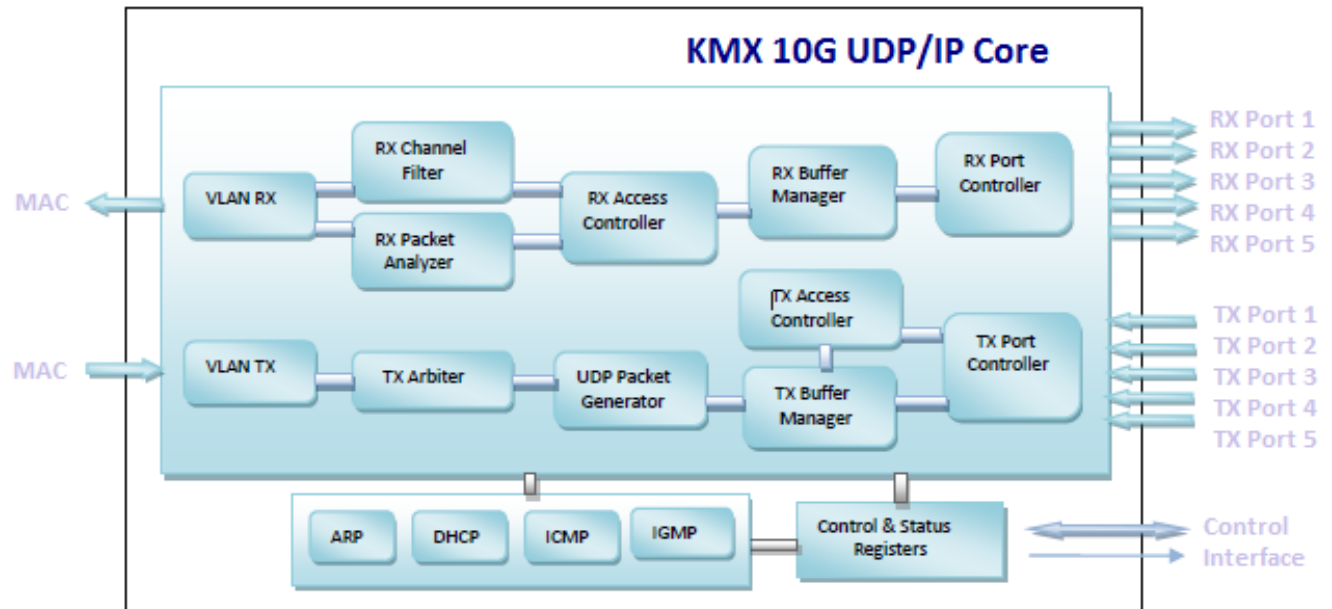
Figure 1 KMX 10G UDP/IP Architecture
